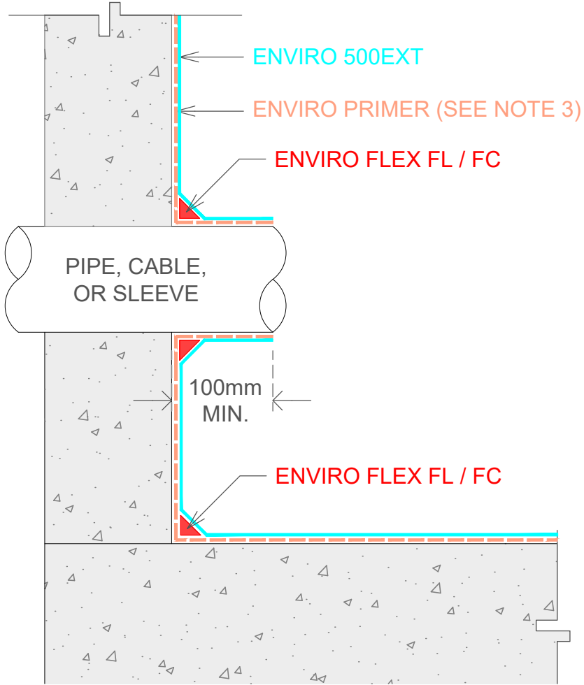
HORIZONTAL WALL PENETRATION DETAIL (PROTECTED)
