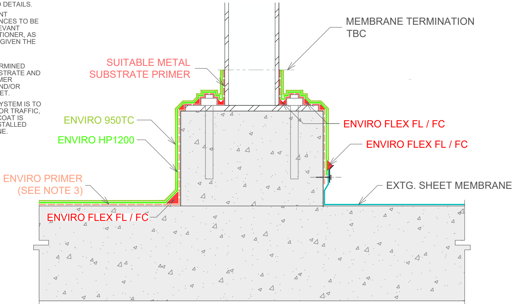
1 HOB DETAIL WITH POST LAPPING ONTO EXISTING MEMBRANE (EXPOSED) SCALE NTS
