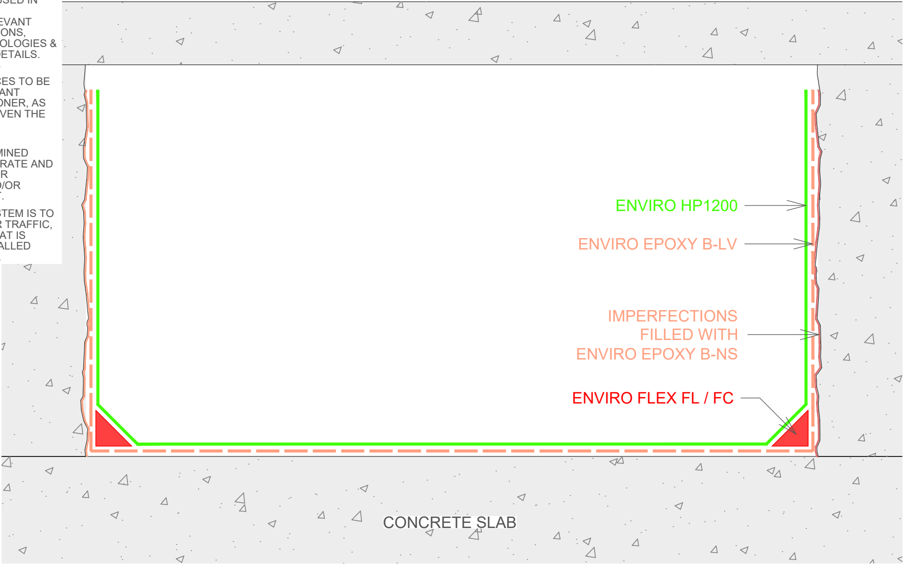
1 OSD/FIRE TANK WITH SUBSTRATE REPAIRS (PROTECTED) SCALE NTS
