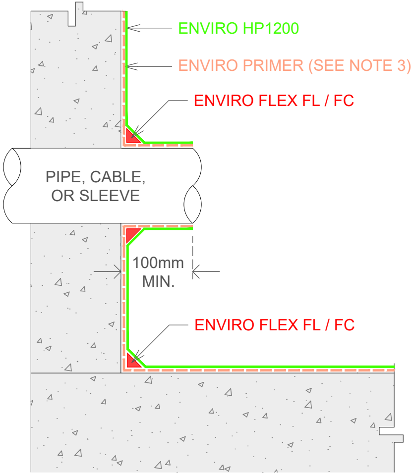
1 HORIZONTAL WALL PENETRATION DETAIL (PROTECTED) SCALE NTS
