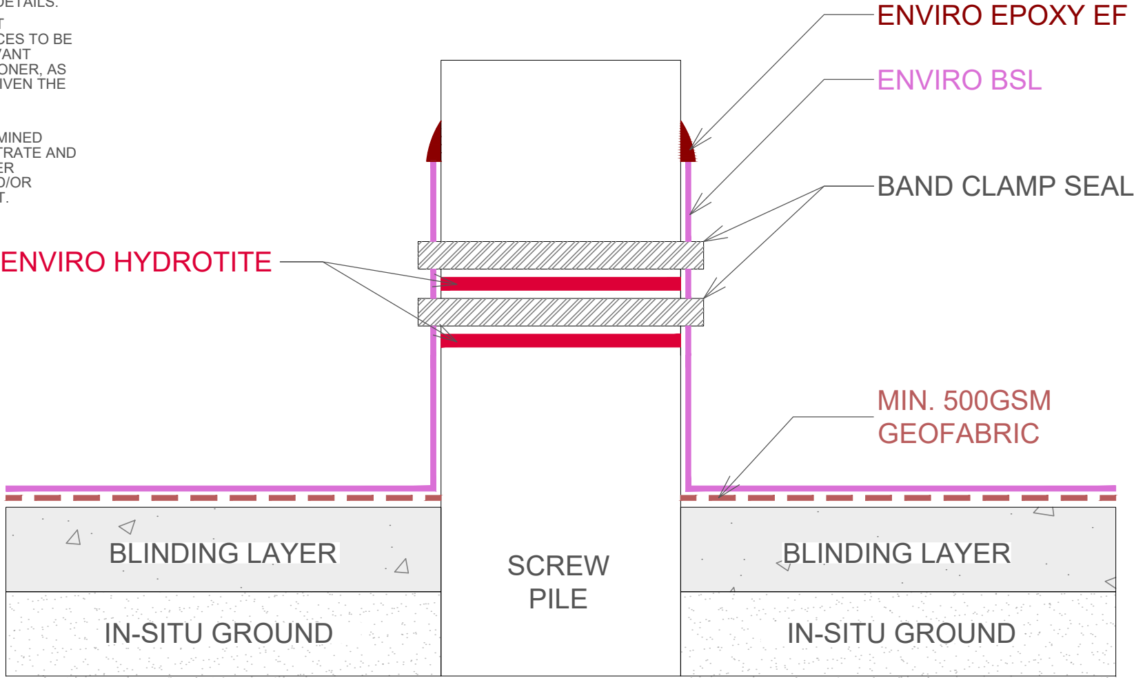
1 PIPE/PILE PENETRATION SCALE NTS
