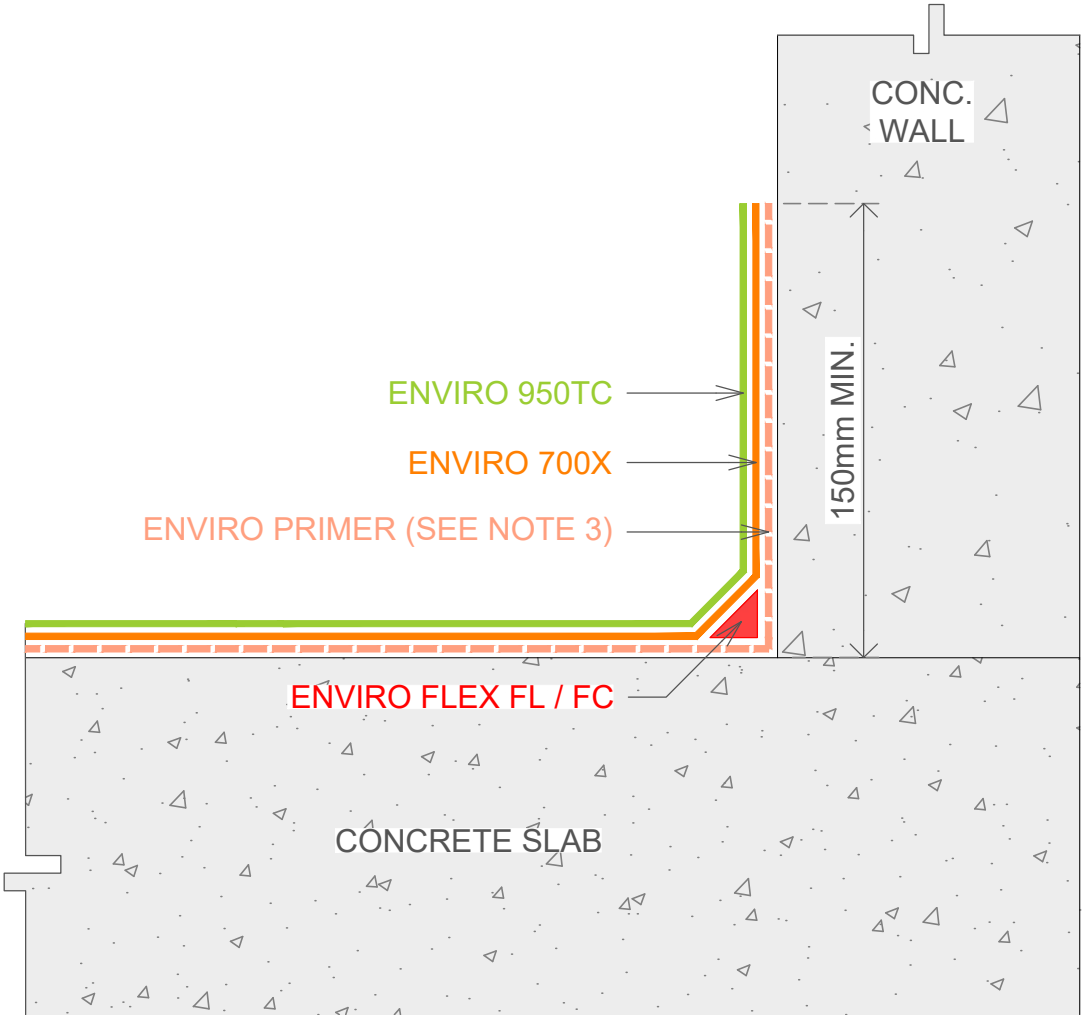
1 UPTURN TERMINATION DETAIL (EXPOSED) SCALE NTS
