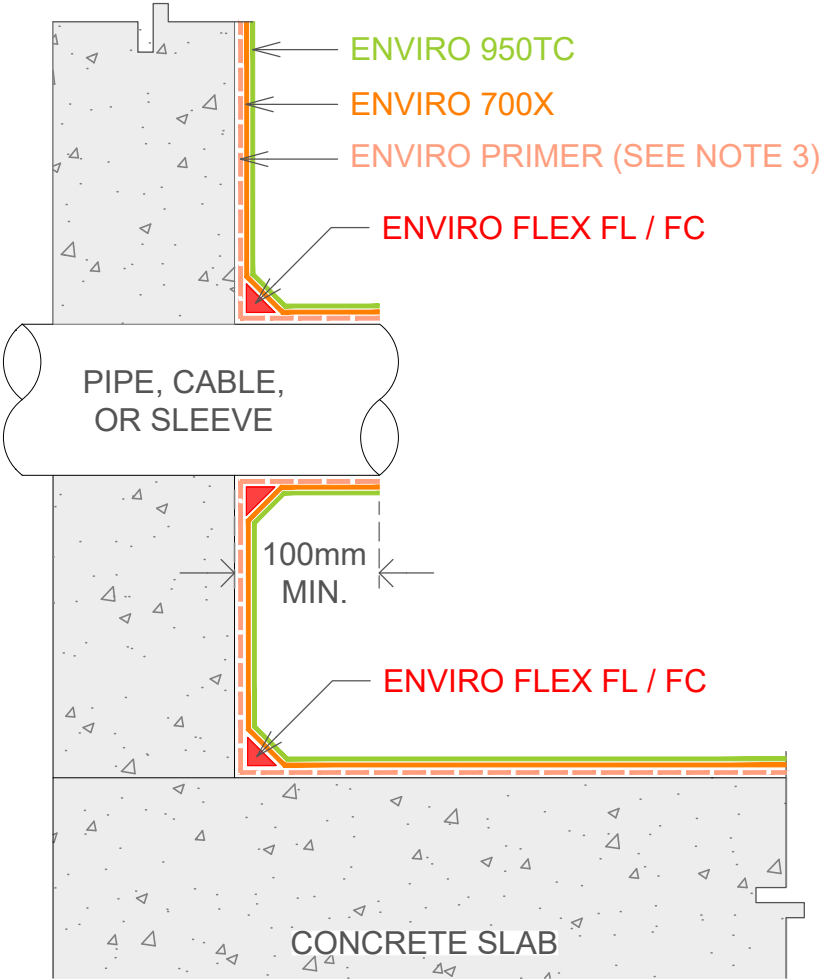
1 HORIZONTAL WALL PENETRATION DETAIL (EXPOSED) SCALE NTS
