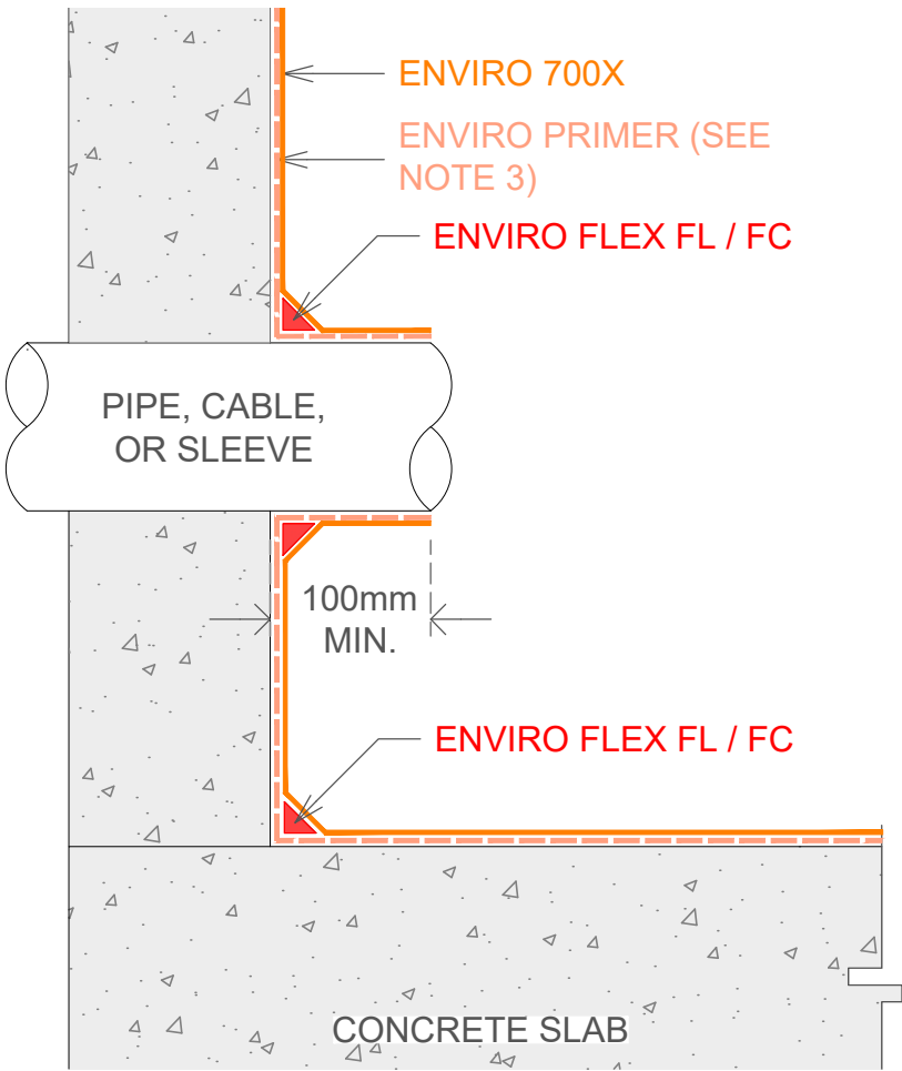
1 HORIZONTAL WALL PENETRATION DETAIL (PROTECTED) SCALE NTS
