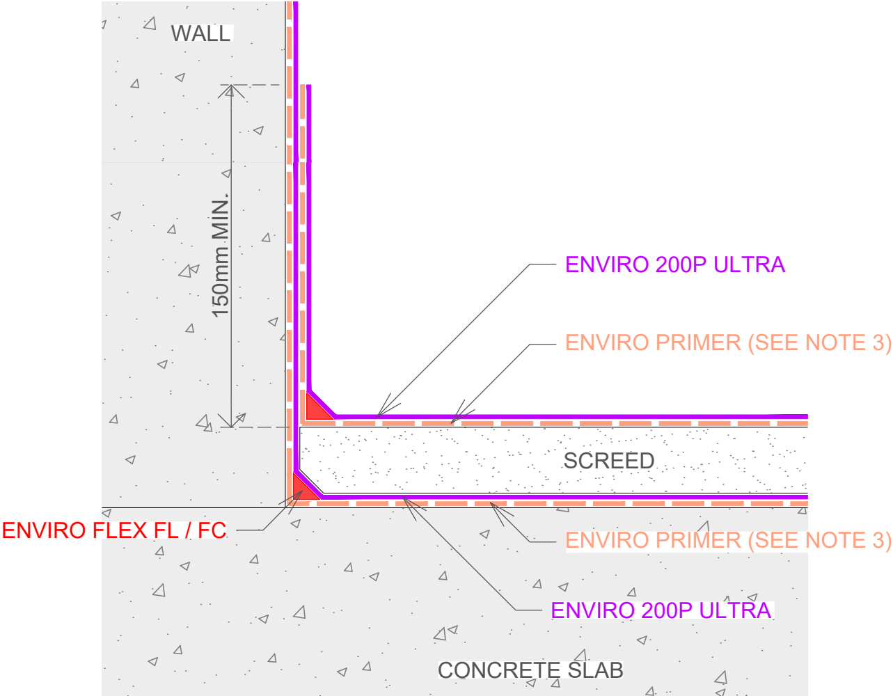
1 DOUBLE INTERNAL WET AREA MEMBRANE DETAIL SCALE NTS
